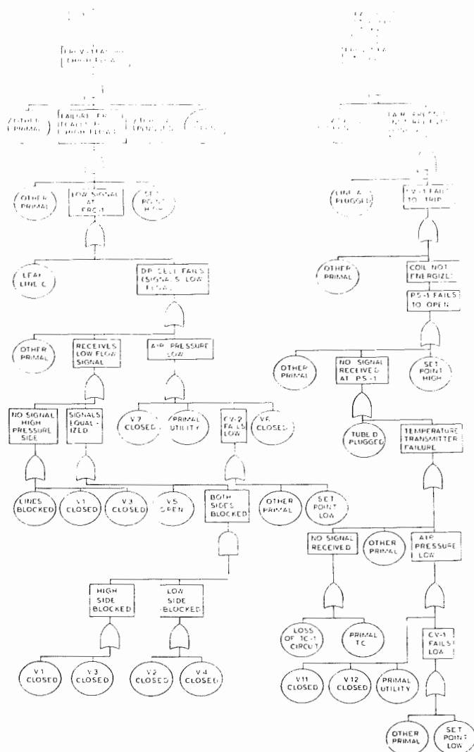
Fig. 3. A fault tree for the system shown in Figure 2. The hazardous event is explosion of the reactor.
