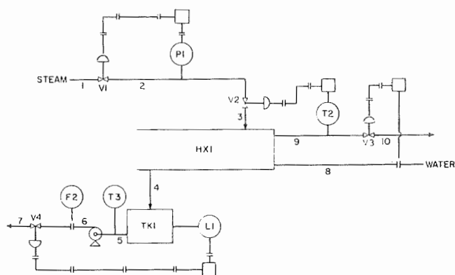
Fig. 9. A model heat exchanger system.
