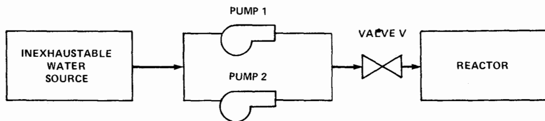
Figure VII-12. Water Pumping System
