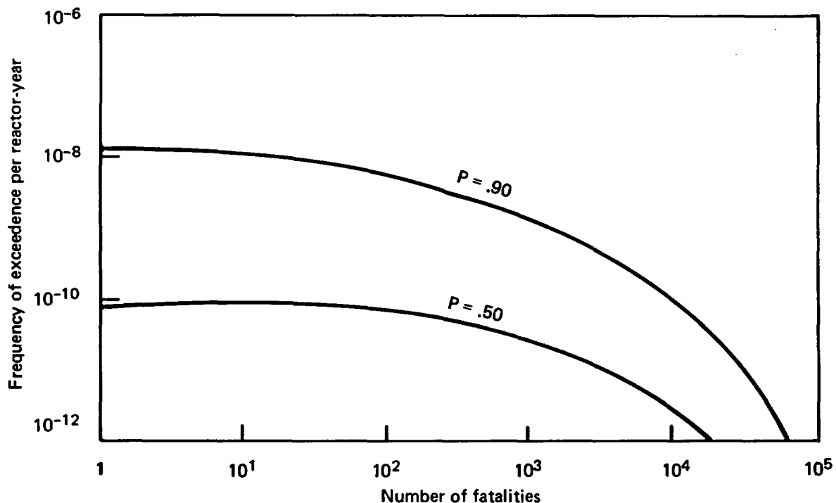
Figure 11-7. Seismic risk curves.
