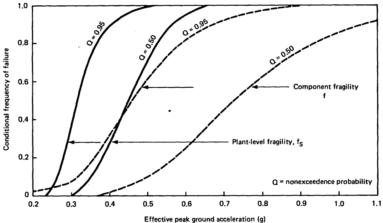
Figure 11-10. Component and plant-level fragility curves.
